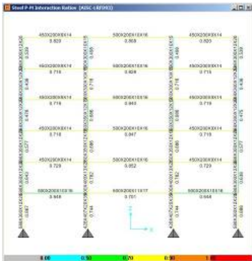
Gambar 14. PM Ratio Portal 2 – 3
