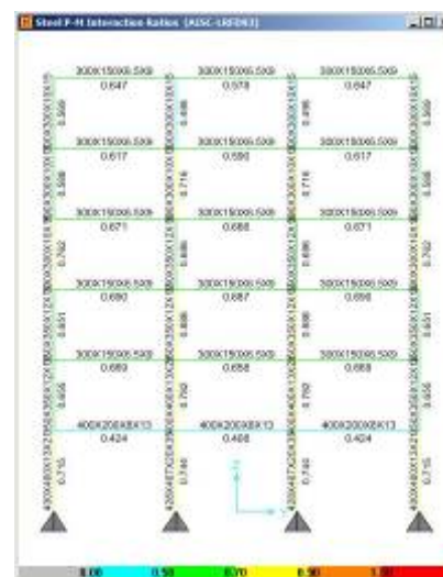
Gambar 13. PM Ratio Portal B - C
